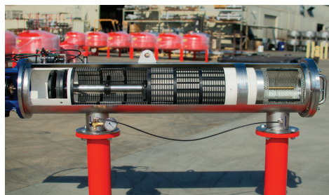
Twist-lock sectional screens provide easy cartridge replacement.
